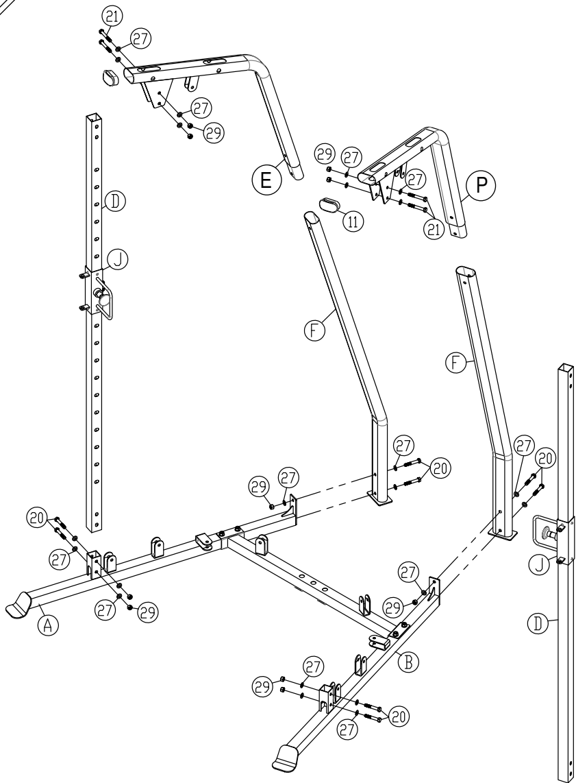
Above shows STEP 2 assembled and completed.
