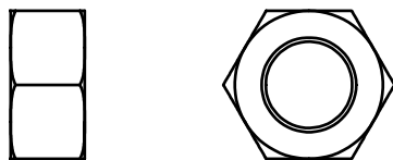
PART 35 - M12 Nut, 1 PCS.
